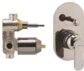
High flow single lever concealed diverter Exposed part F1018721GG ₹ 4,540 Concealed part F4030101GG ₹ 5,620 Set ₹ 10,160
